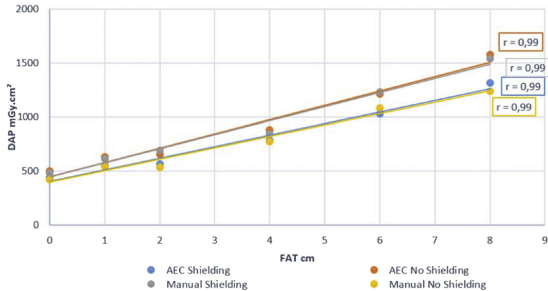
Figure 10. DAP with/without shielding – AEC and Manual exposure.
